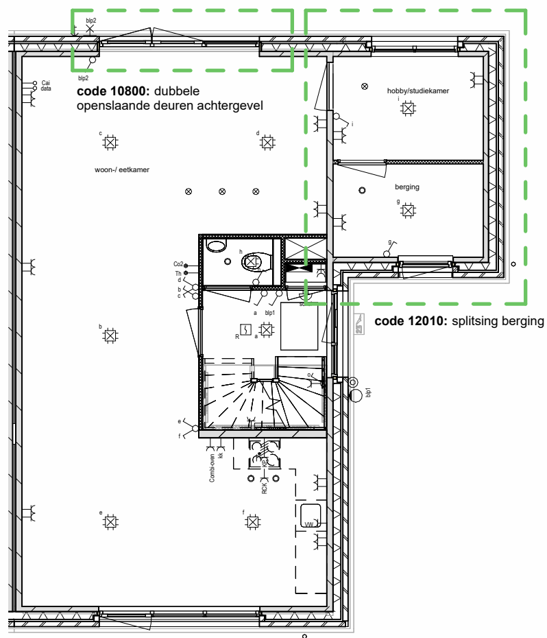
00 begane grond
