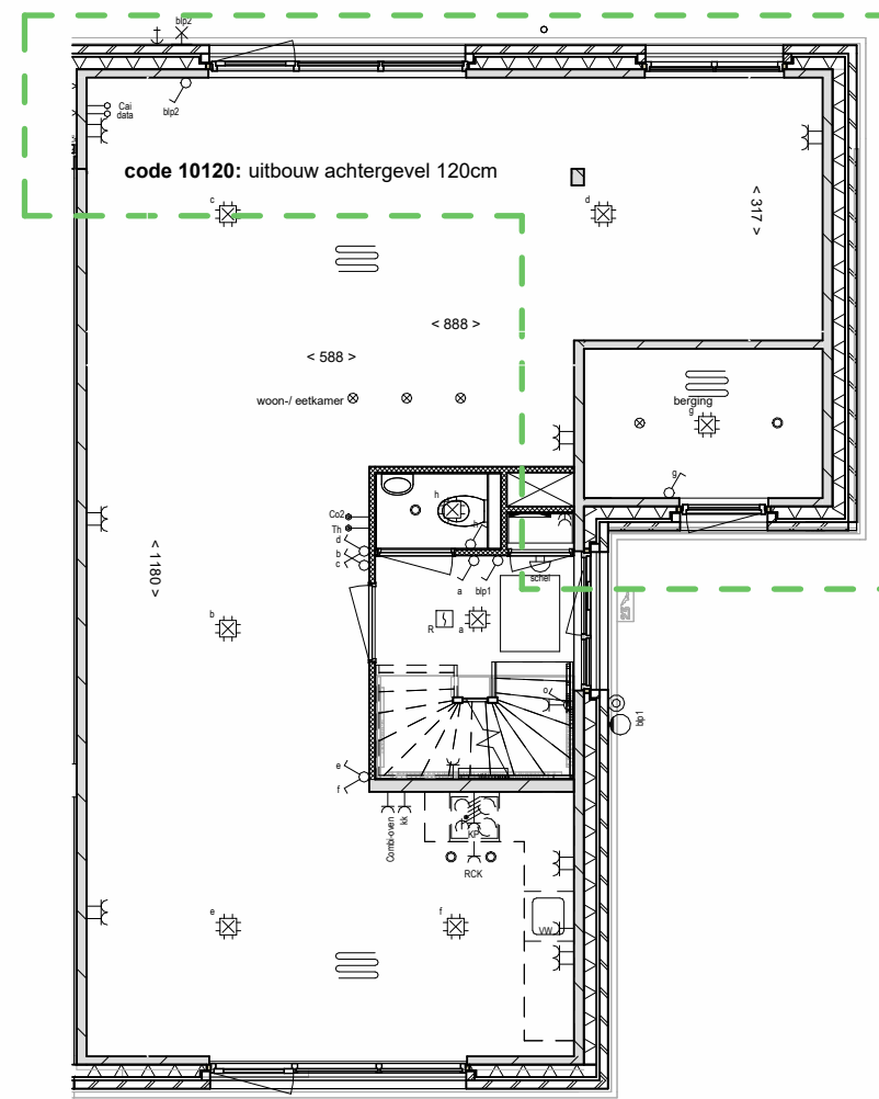
00 begane grond
