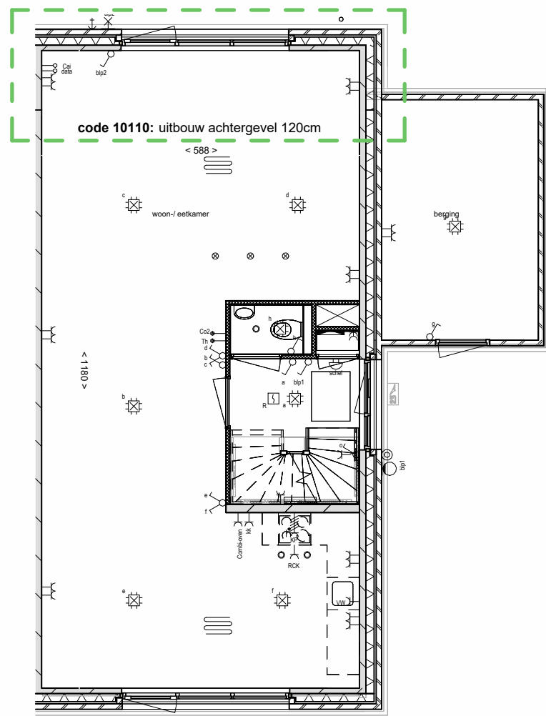
00 begane grond
